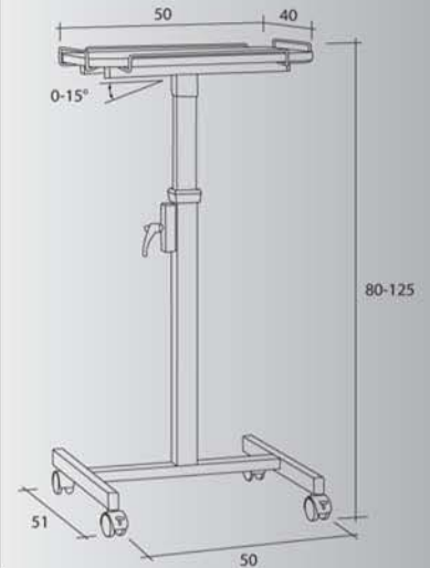
Portable A.V. Table Model no. 49465 Tilt adjustment for projection tray and telescopic height adjustment
