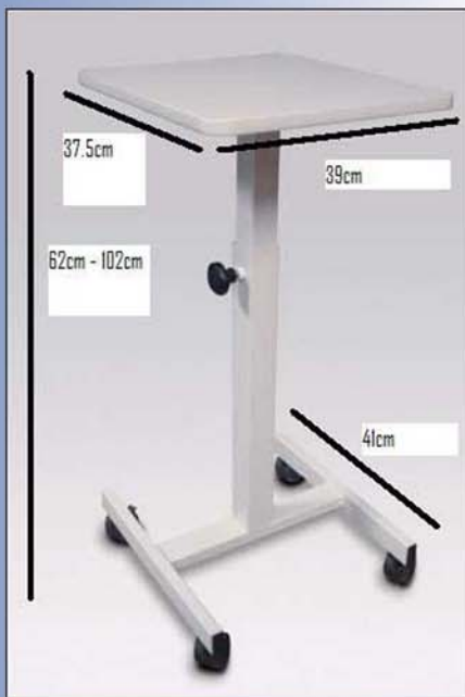
49483 Standard AV trolley Height adjustment 62-102cm. Shelf size 37.5 x 39cm. 4 castor wheels, 2 lockable. Max load 20 kgs. K.D. shipping weight 7.5 kgs.
